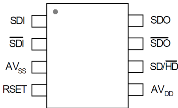
Figure 1 – M08018 Pin-out diagram
