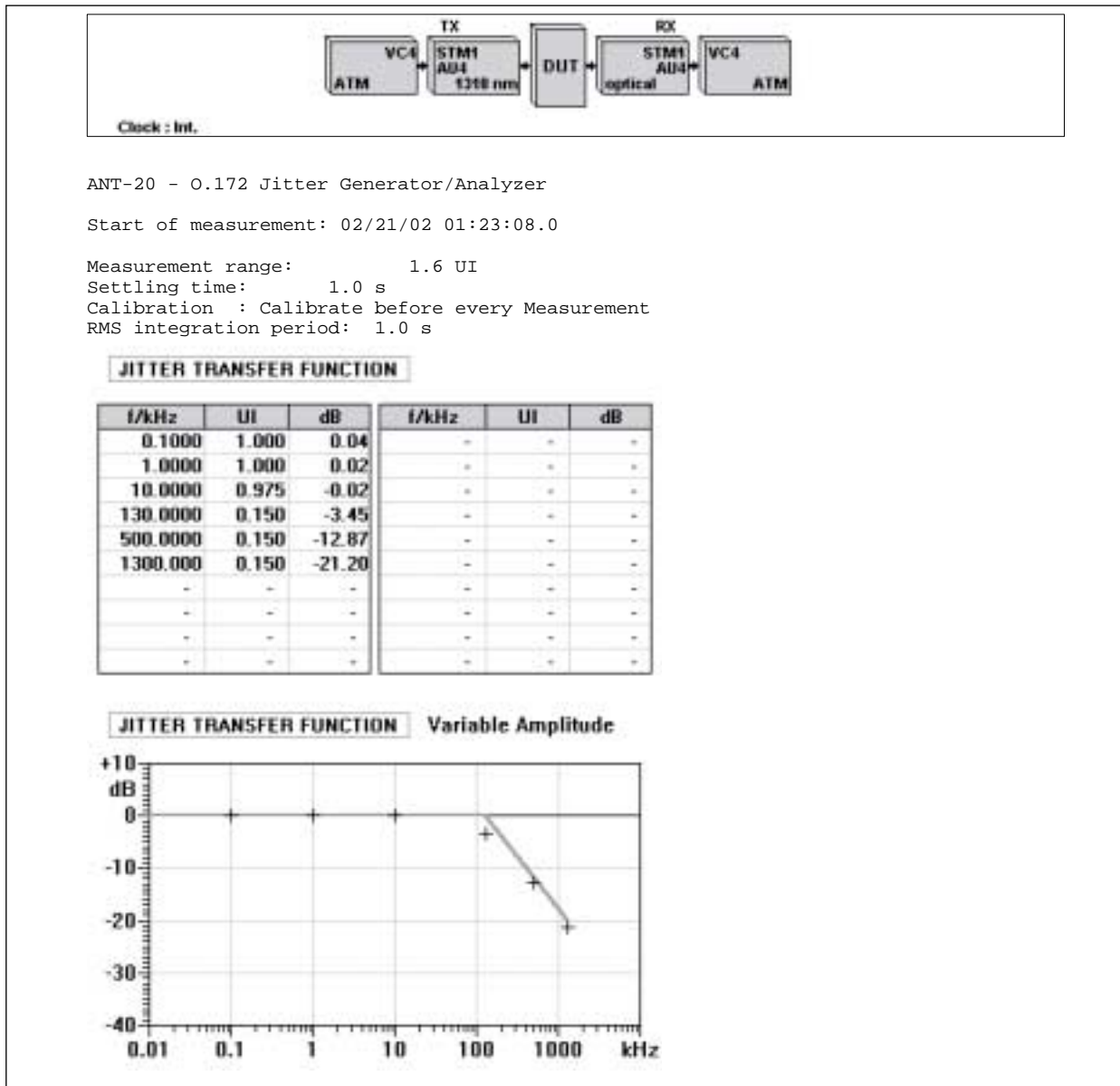
Figure 4. Jitter Transfer, Loop Timed
