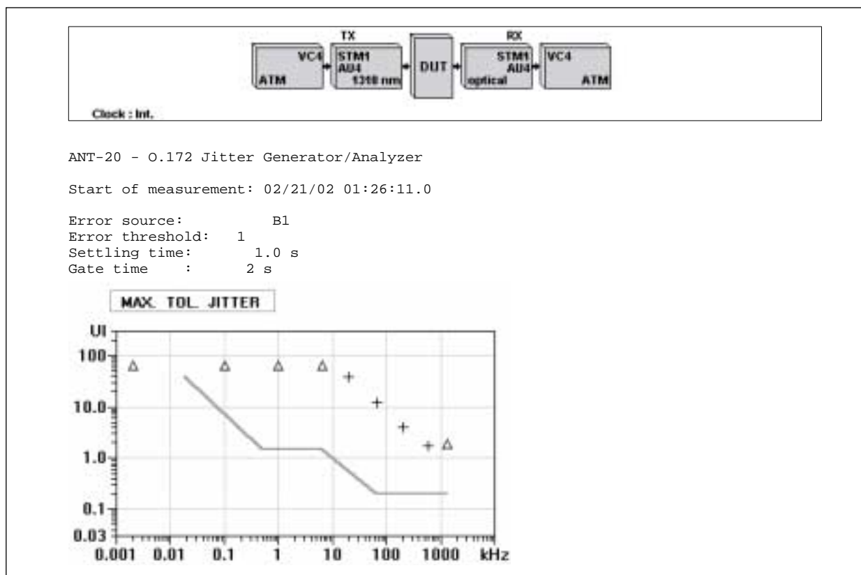
Figure 1. Jitter Tolerance, Loop Timed
