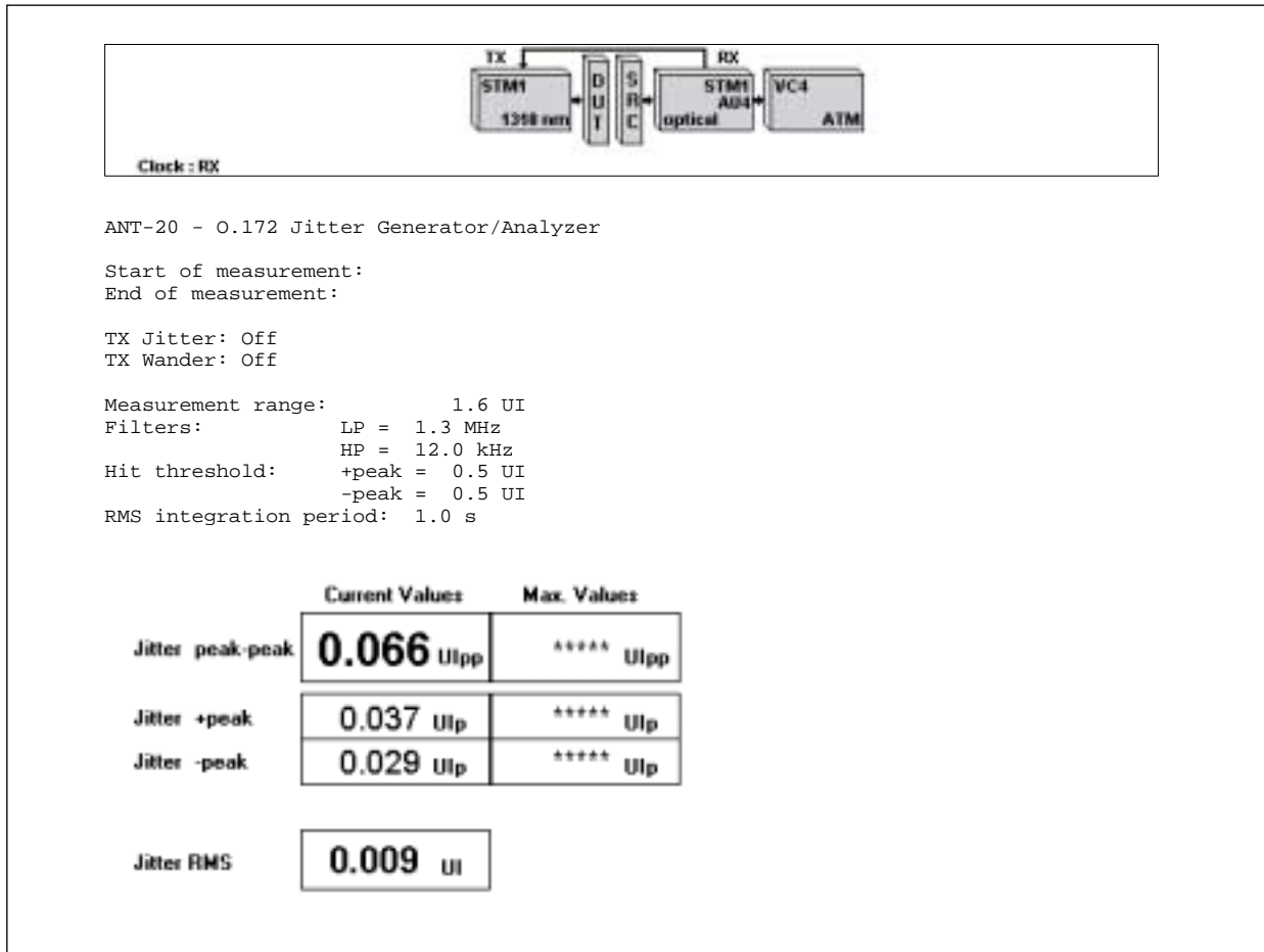
Figure 3. Intrinsic Jitter, Loop Timed
