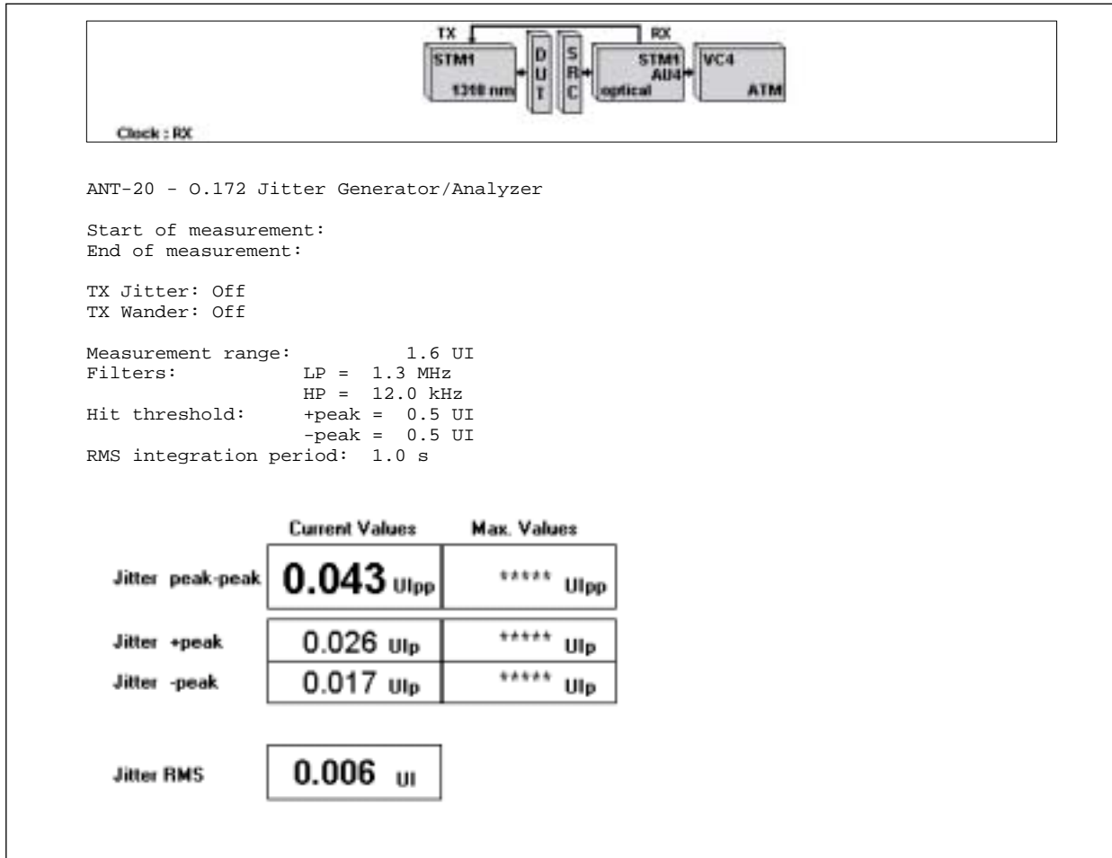
Figure 2. Intrinsic Jitter, System Timed
