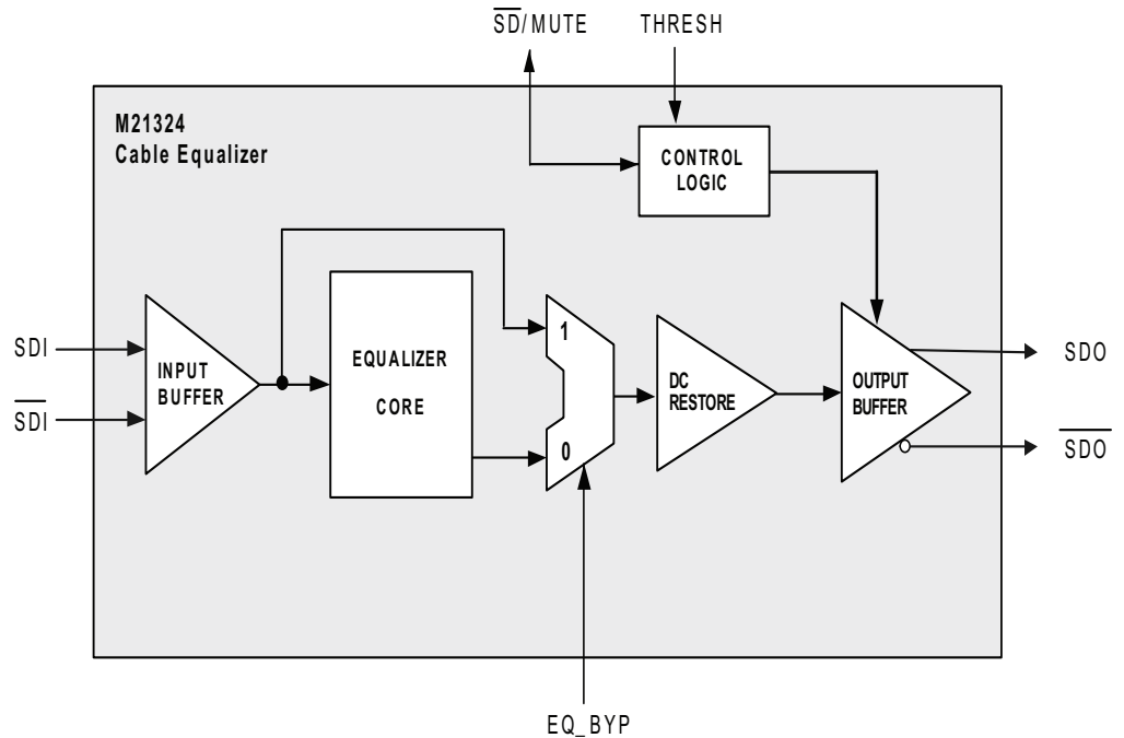
Fig. 2 - Block Diagram (M21324 Cable Driver)
