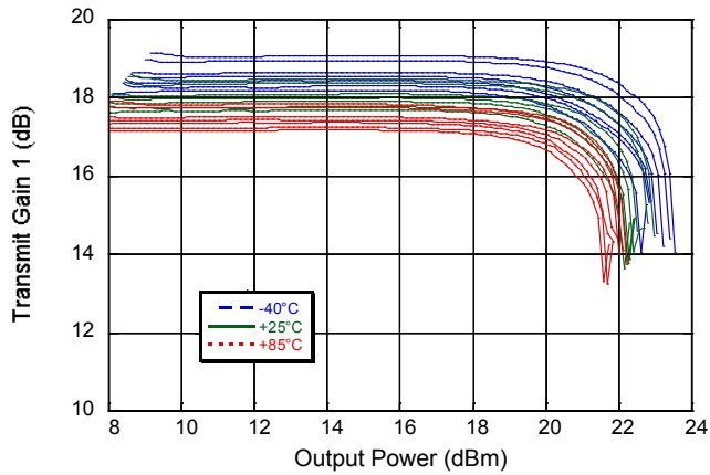
Gain_TX1
