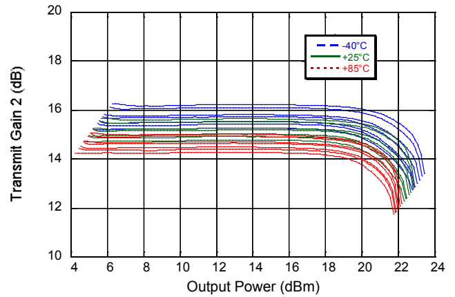
Gain_TX2
