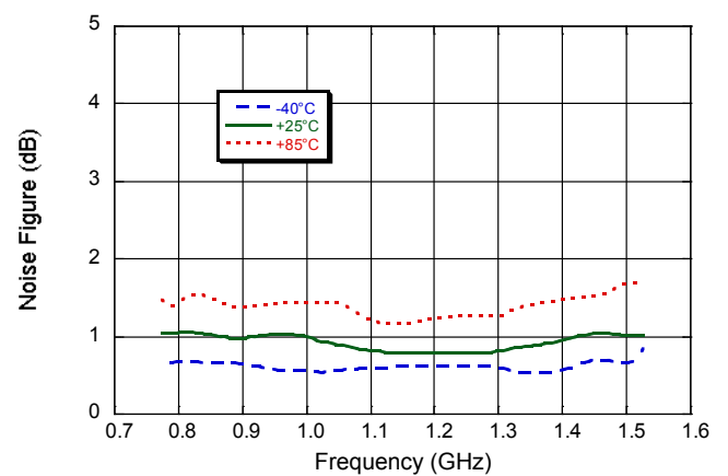
Noise Figure
