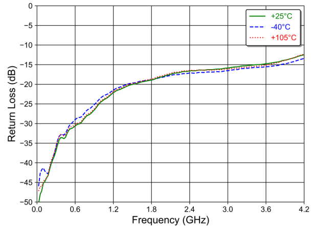
RF4 Return Loss 9 , RFCOM-RF4
