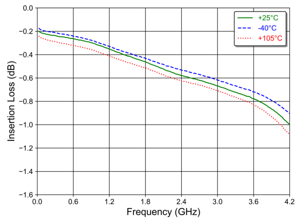
Switch Insertion Loss 9 , RFCOM-RF4
