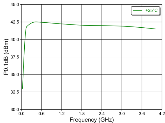
Compression P0.1dB 9
