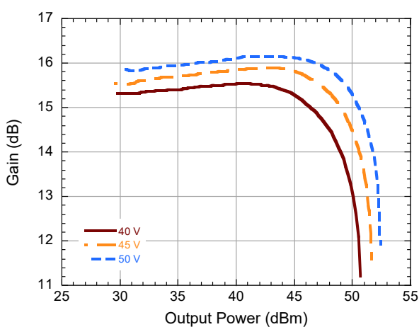
Gain vs. Output Power and V_{DS}
