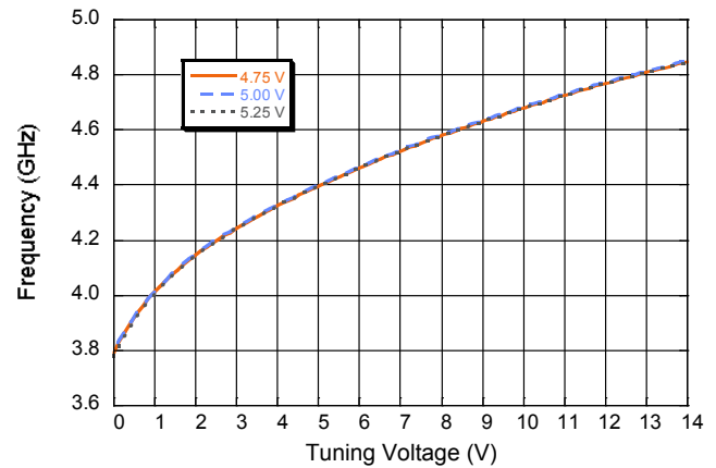
Output Frequency vs. Tuning / Supply Voltage - RF/2 Port
