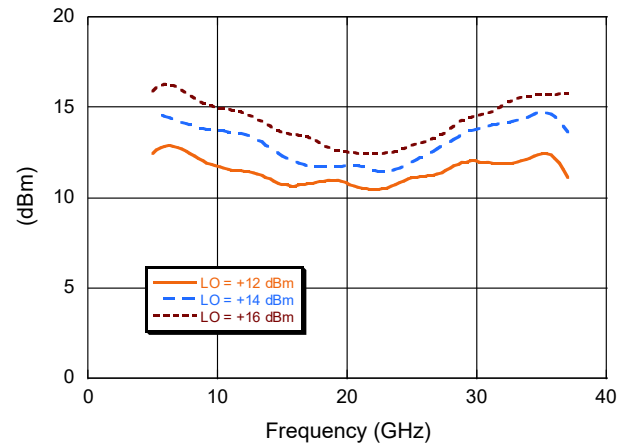
Input P1dB (Down Conversion)
