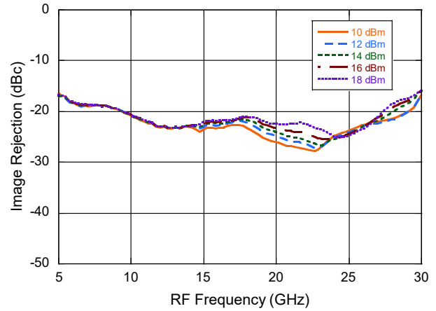
Up Conversion SSB (USB) over LO Drive
