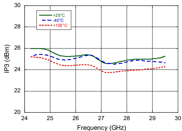
RX IP3
