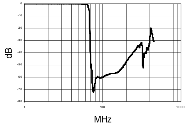
Common to MoCA Path filter performance
