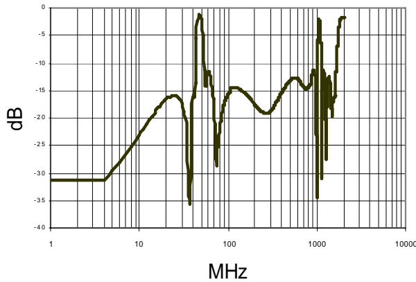
Common to Forward Path filter performance
