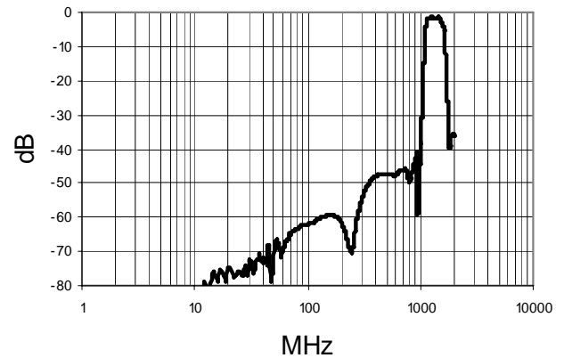
Common to MoCA Path filter performance
