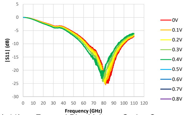
|s_{11}| vs. Forward Bias Voltage, Series Connection, W Band, MADZ-011002
