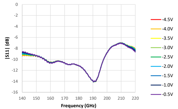
|s_{11}| vs. Reverse Bias Voltage, Series Connection, G Band, MADZ-011002
