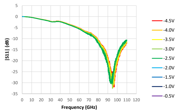
|s_{11}| vs. Reverse Bias Voltage, Series Connection, W Band, MADZ-011002
