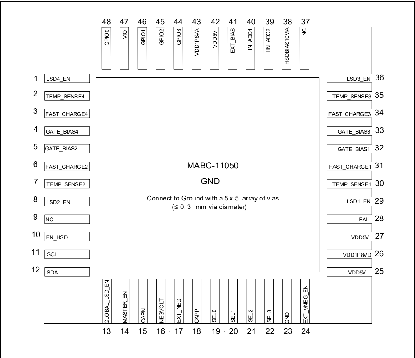
Figure 2-1. MABC-11050 Pinout
