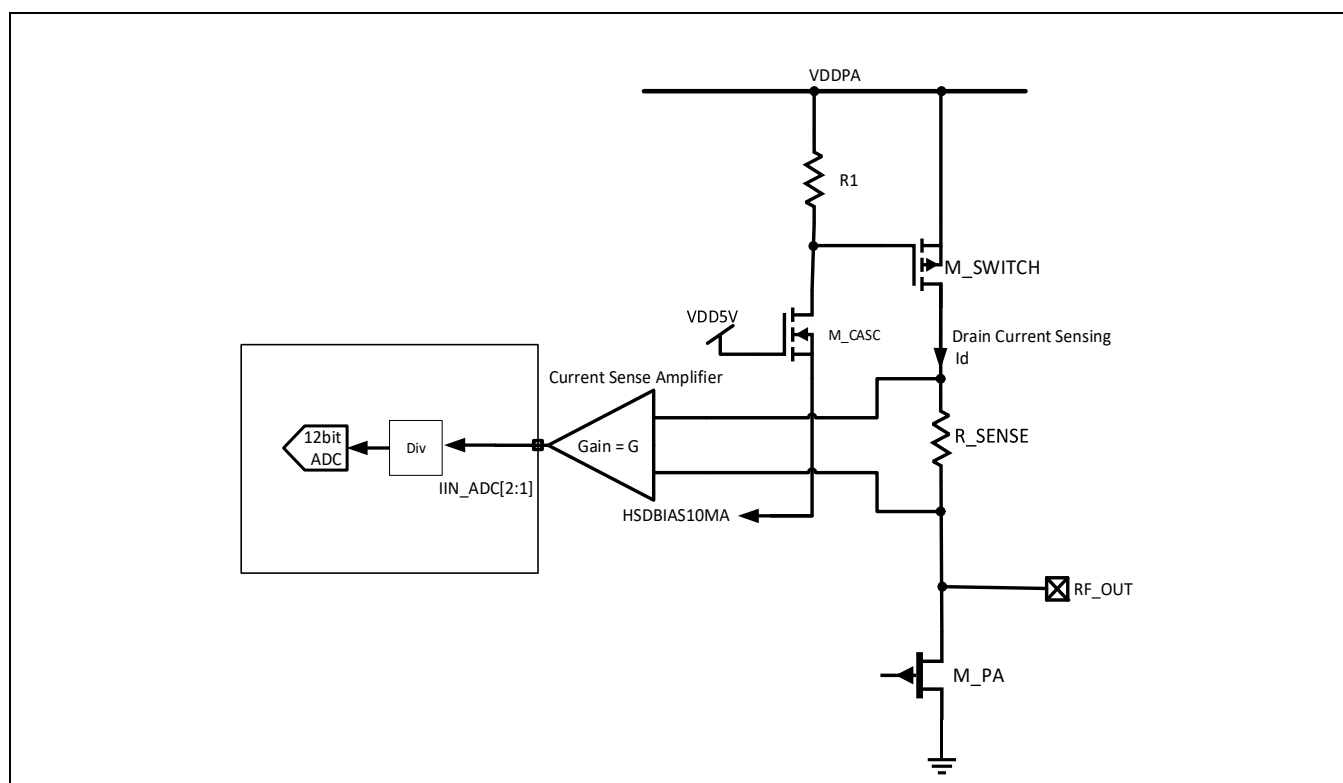
Figure 3-8. Drain Current Sensing Block Diagram
