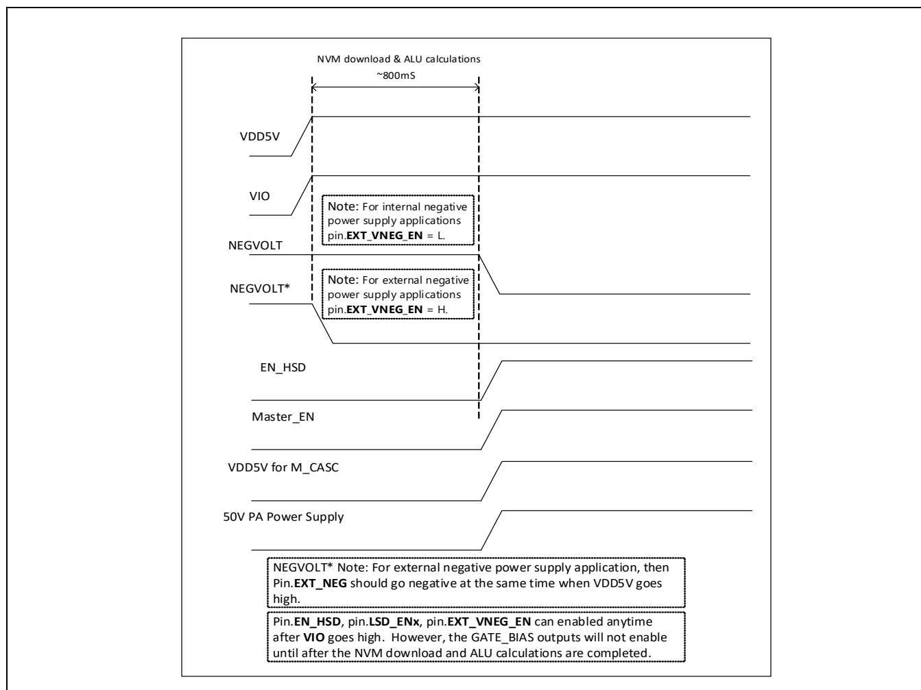
Figure 3-2. Power-up Sequencing
