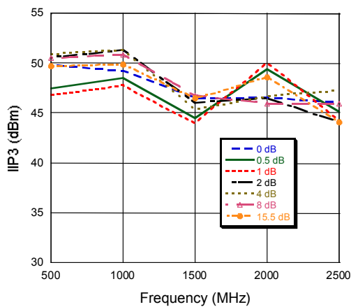
IIP3, +5 V, vs. Attenuation Setting
