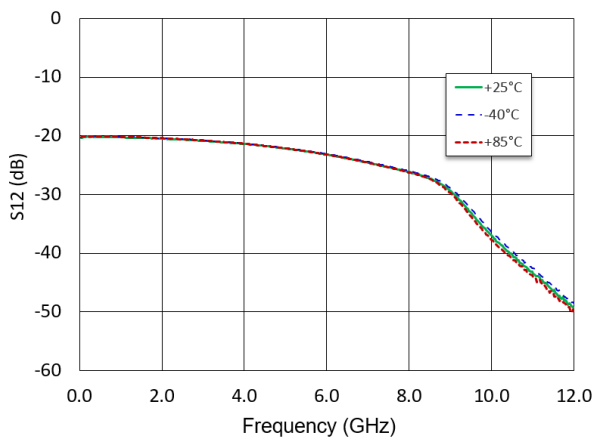
Reverse Isolation
