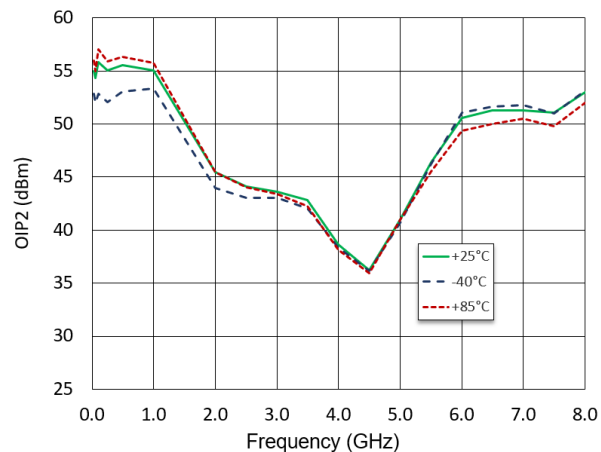
OIP2 at P_{IN} = -15 dBm/tone, 6MHz Spacing
