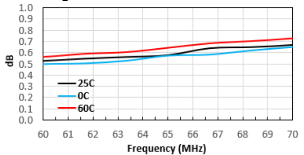
Noise Figure
