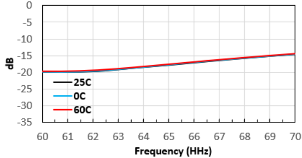
Output Return Loss
