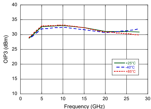
Output IP3 (10 MHz Tone Spacing, P_{IN} = -5\text{ dBm} per tone)
