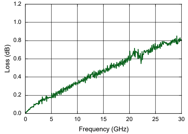
Test Board Line Loss, 1 port loss
