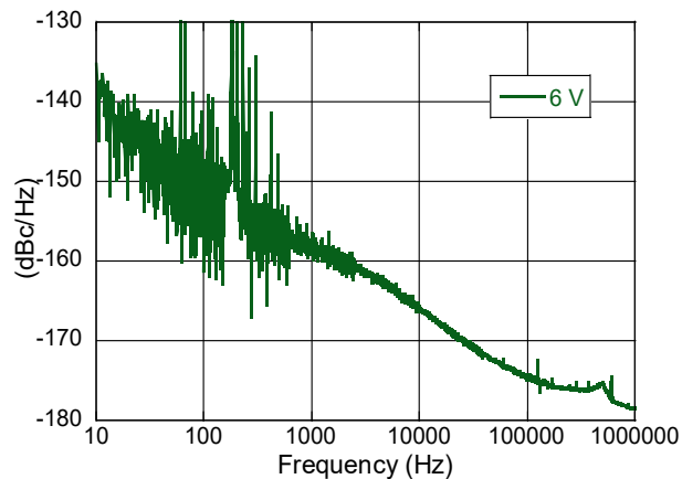
Phase Noise @ 10 GHz, P3dB
