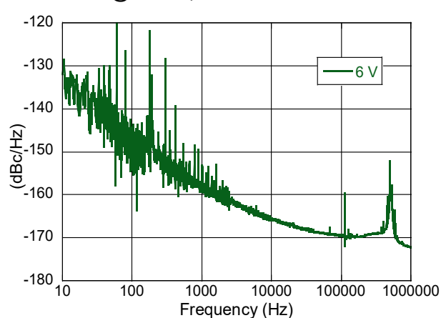
Phase Noise @ 20 GHz, P3dB
